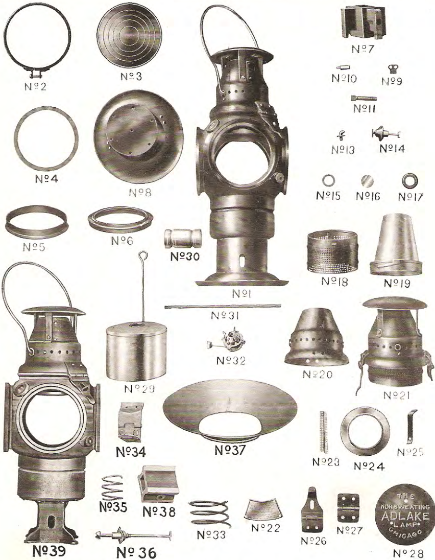
Parts of No. 169 and No. 169 \frac{1}{2} Switch Lamp
